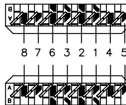
KROME CONNECTOR PIN ASSIGNMENT
